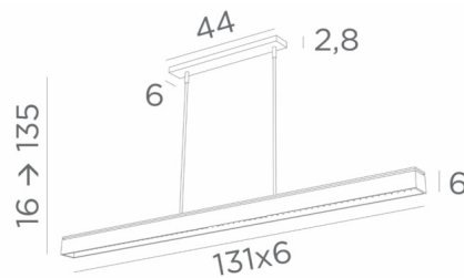
GALAND J tubes in brushed bronze. Metal finish code: 29
