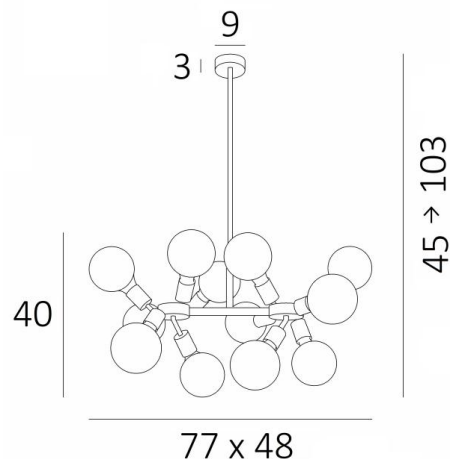
OURIS 2 in brushed bronze with silver bulbs Ø125mm. Metal finish code: 29
