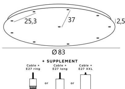
CEILING BASE 10 ø83 in structured black. Metal finish code: 02. Optional: a wide choice of cables and fittings (+supplement)
