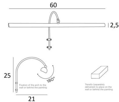
TRIANON 60 in brushed nickel. Metal finish code: 33
