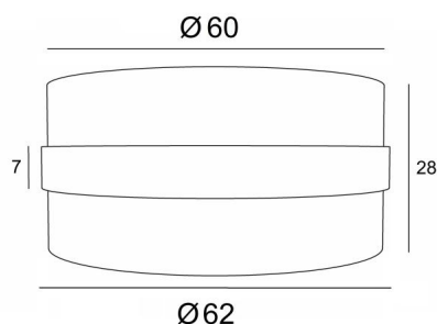
Lampshade TOUYA 60 in Turda Blond (fabric from category 3) with ring in Turda Abricot
