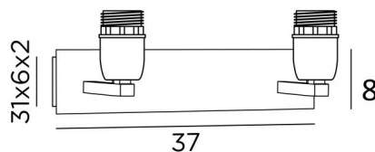
MONTOU in brushed bronze without lampshades
