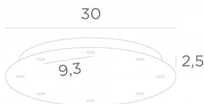
Ceiling base 8 ø30
